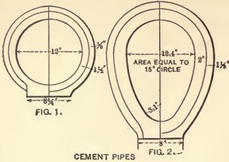
CEMENT PIPES
